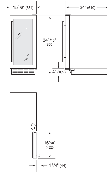
Dimensions based on stainless steel model.
