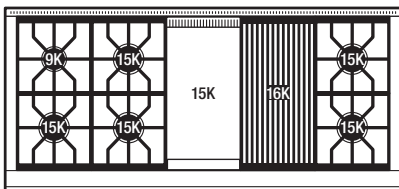
60" Gas Range – 6 Burners, Infrared Charbroiler and Infrared Griddle
