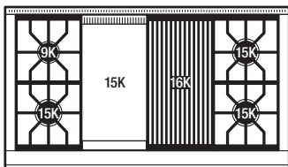
48" Gas Range – 4 Burners, Infrared Charbroiler and Infrared Griddle
