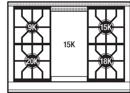
36" Sealed Burner Rangetop – 4 Burners and Infrared Griddle
