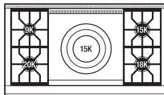
48" Sealed Burner Rangetop – 4 Burners and French Top
