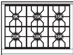
36" Dual Fuel Range – 6 Burners
