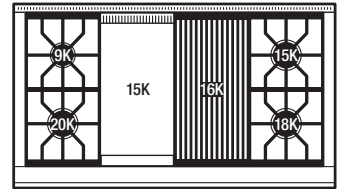
48" Dual Fuel Range – 4 Burners, Infrared Charbroiler and Infrared Griddle
