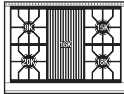
36" Sealed Burner Rangetop – 4 Burners and Infrared Charbroiler
