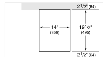
COUNTERTOP CUT-OUT
